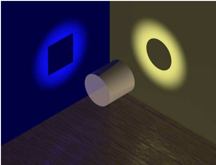
PICTURE 6 - A GEOMETRICAL METAPHOR FOR THE DUALITY WAVE PARTICLE
